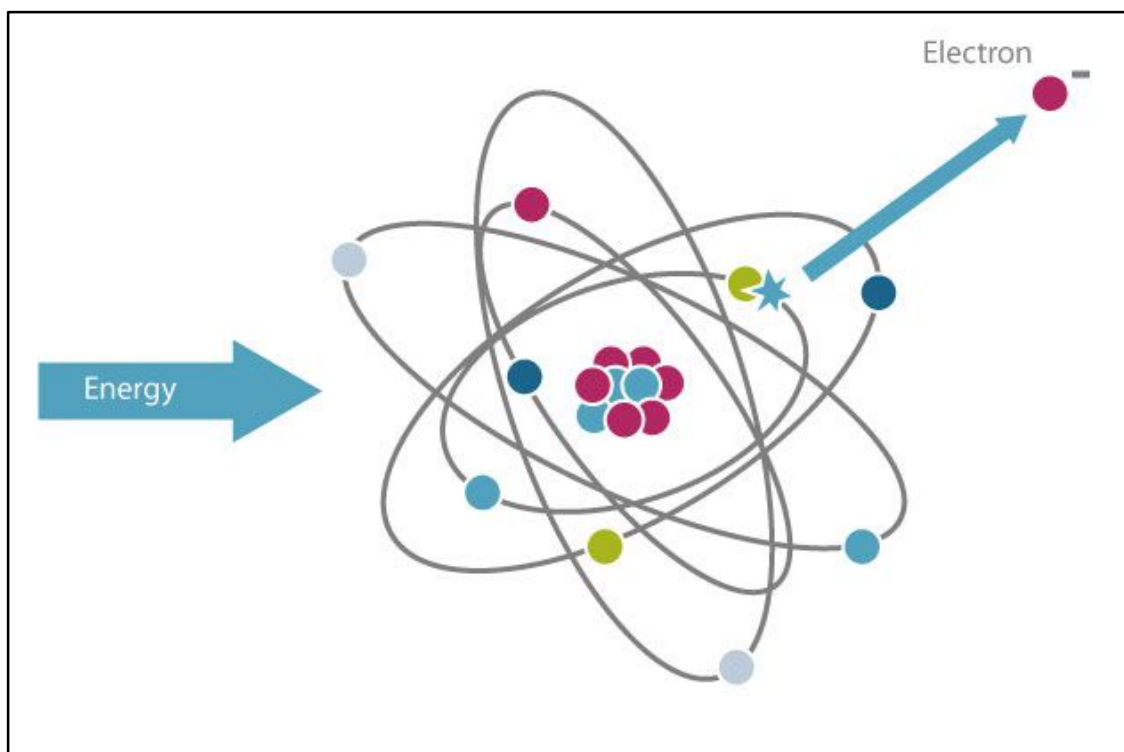
Fig. 1. Knocking of electron from an atom due to exposure to ionizing radiation atom.
