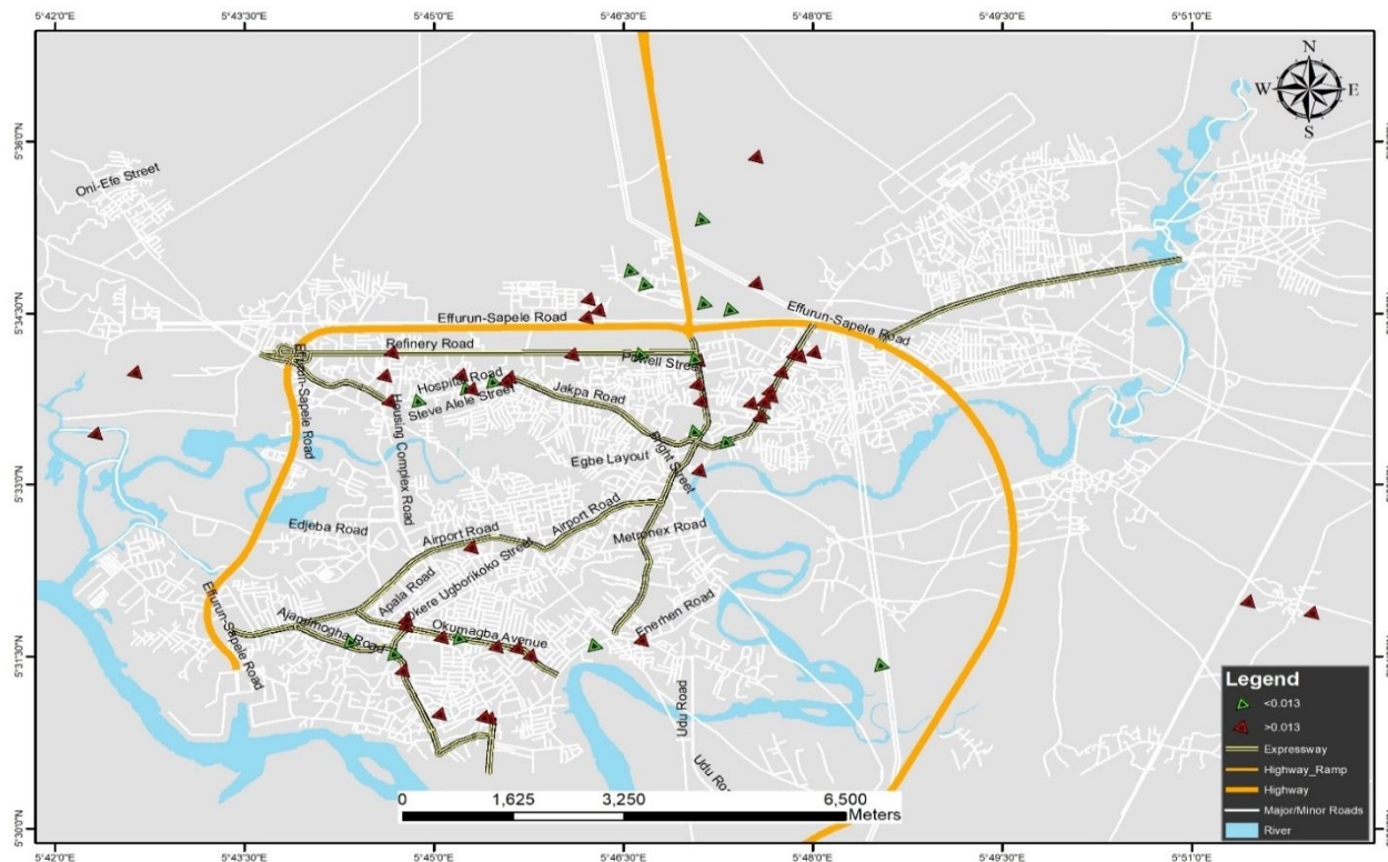
Fig. 3. GIS map of the sampled area showing sampled points with BIR exposure rate within and above world normal BIR level ( 0.013\text{mRh}^{-1} ).
