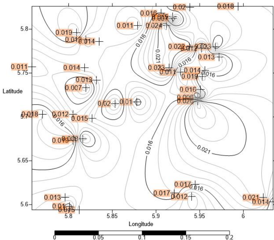
Fig. 2. GIS contour map of the study area showing sampled points with BIR exposure rate.
